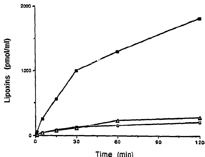
Fig. 4. Time-course of the conversion of exogenous 5(S),6(R)-diHETE ( 10 \mu\text{M} ) to lipoxins in human platelets. The incubations were performed at 37^\circ\text{C} in the presence of A23187 ( 1 \mu\text{M} ). ( \blacksquare ) \text{LXA}_4 ; ( \Delta ) 11- trans - \text{LXA}_4 ; ( \circ ) peak I (cf. Fig. 1).
